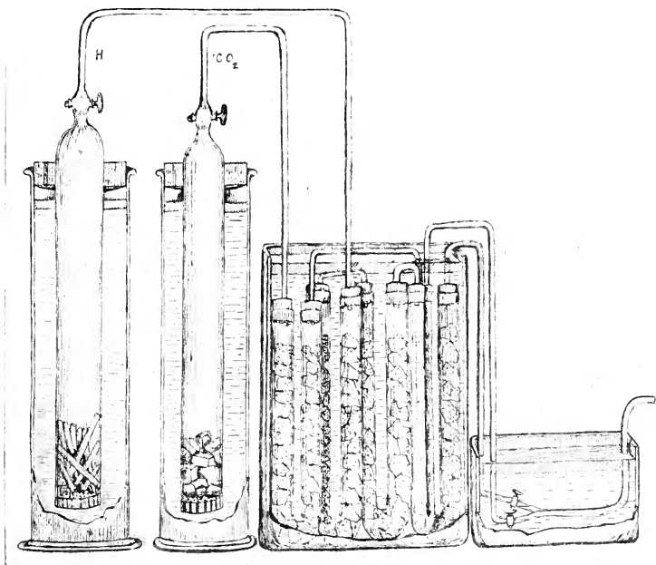
FIG. 58. Apparatus for obtaining pure hydrogen and pure carbon dioxide free from all oxygen. All the connexions are submerged in water, and all the liquids are covered with a layer of liquid paraffin. (The generators one-tenth and the remaining apparatus one-sixth natural size. After Ewart.)
